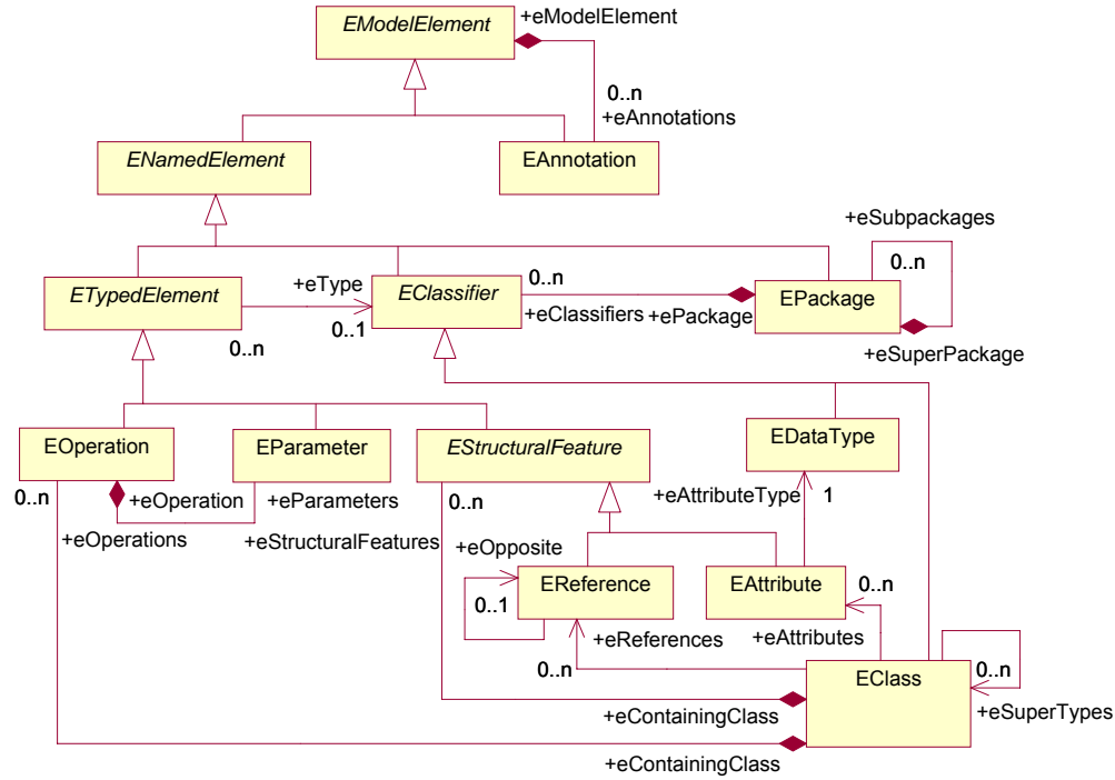
Figure 3: Kernel of Ecore model
