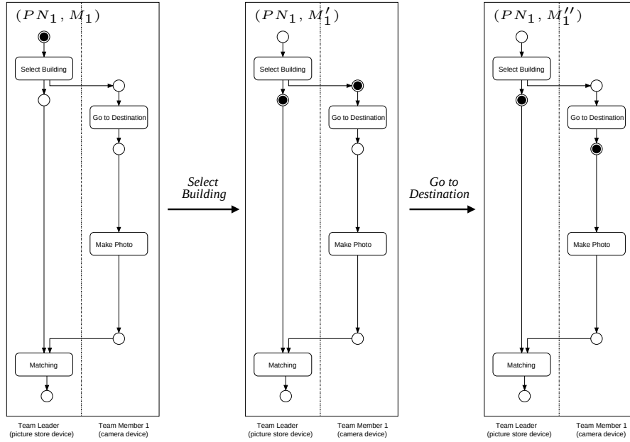
Figure 1. Cooperative process of the team and firing steps Select Building and Go to Destination
