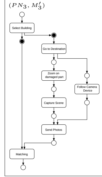
Figure 6. P/T-system (PN_3, M_3')
