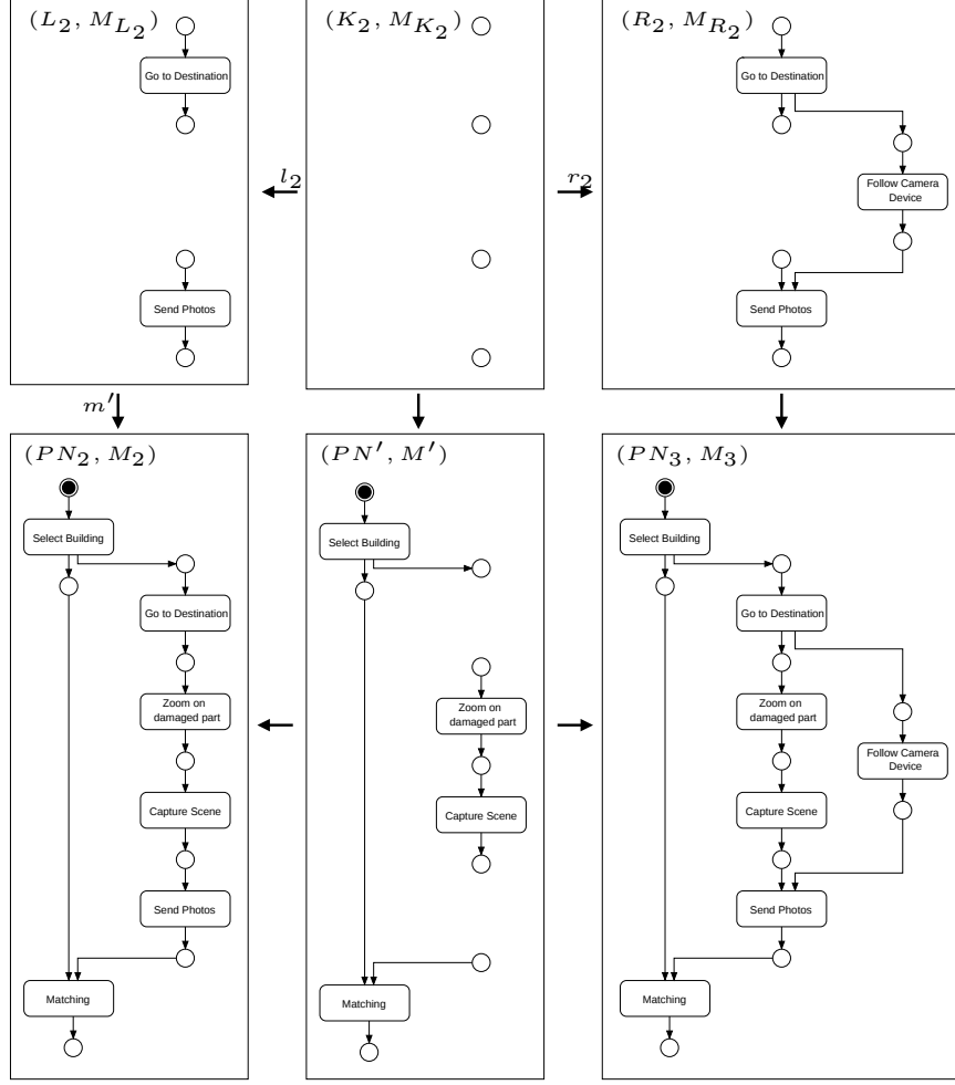
Figure 3. Transformation step (PN_2, M_2) \xrightarrow{prod_{follow, m'}} (PN_3, M_3)
