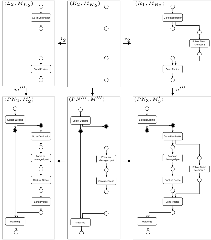
Figure 7. Transformation step (PN_2, M_2') \xrightarrow{prod_{follow}, m'''} (PN_3, M_3')
