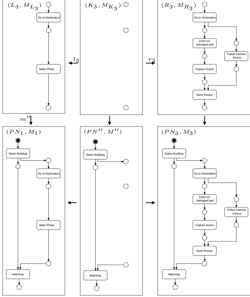
Figure 5. Direct transformation of (PN_1, M_1) via the concurrent rule prod_{conc}
