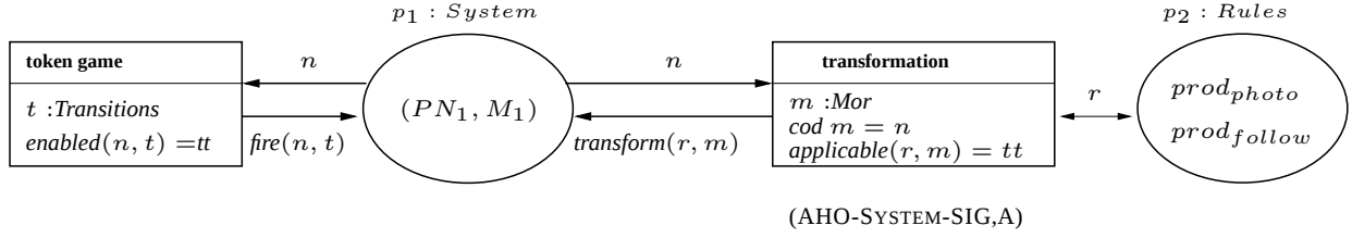
Figure 10. Algebraic higher-order system
