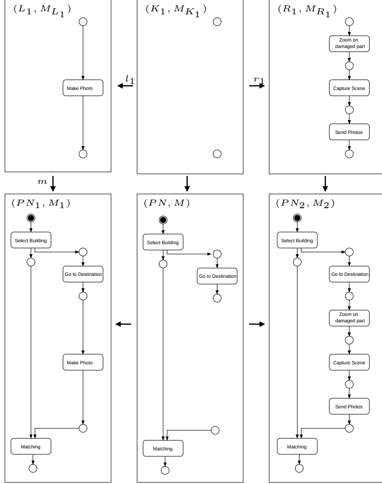
Figure 2. Transformation step (PN_1, M_1) \xrightarrow{prod_{photo.m}} (PN_2, M_2)
