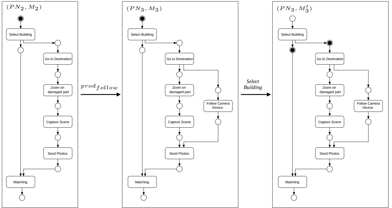
Figure 9. Pair of steps ((\text{prod\_follow}, m', n'), \text{Select Building})
