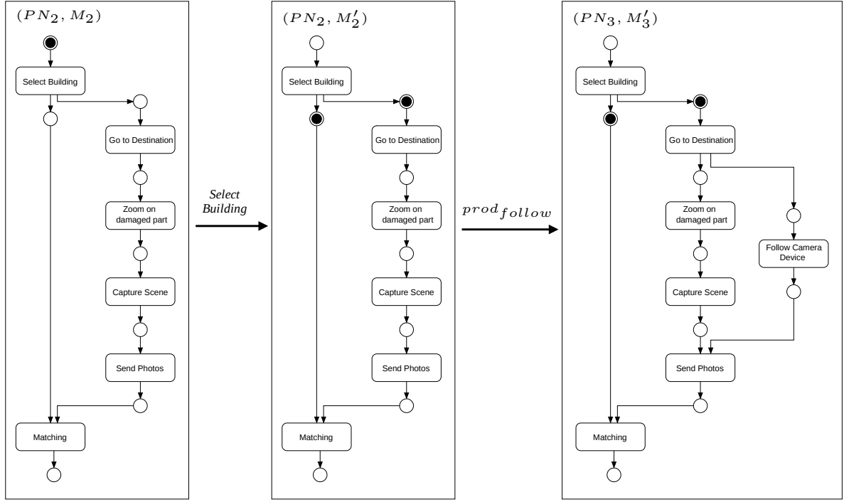
Figure 8. Pair of steps (\text{Select Building}, (\text{prod\_follow}, m''', n'''))
