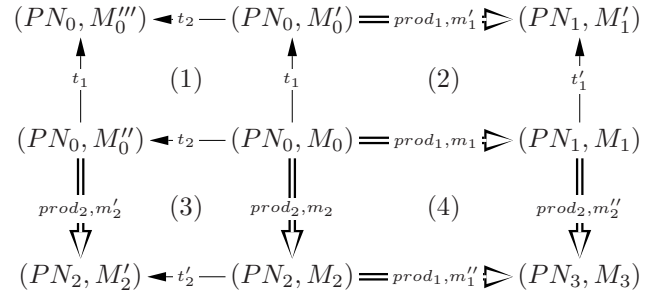
Figure 4. Concurrency in reconfigurable P/T systems
