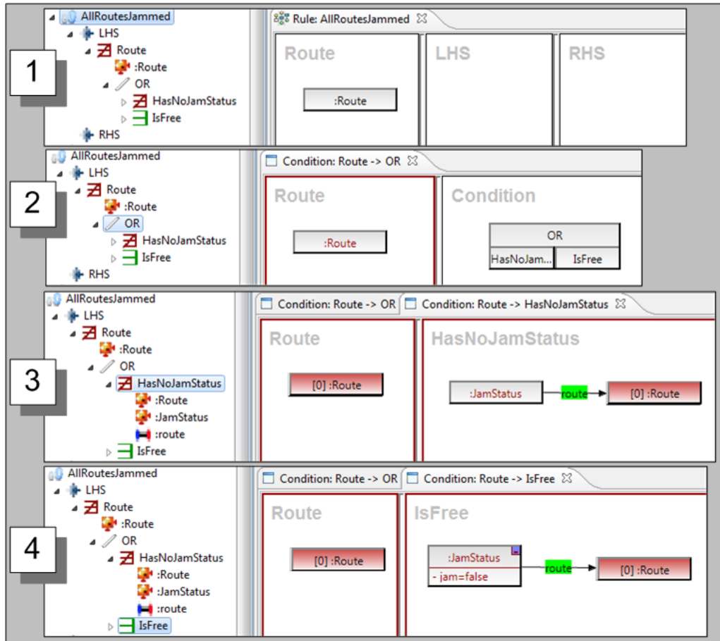
Figure 7: Empty rule AllRoutesJammed with application condition
