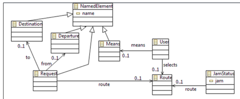
Figure 3: Meta-model for the Personal Mobility Manager
