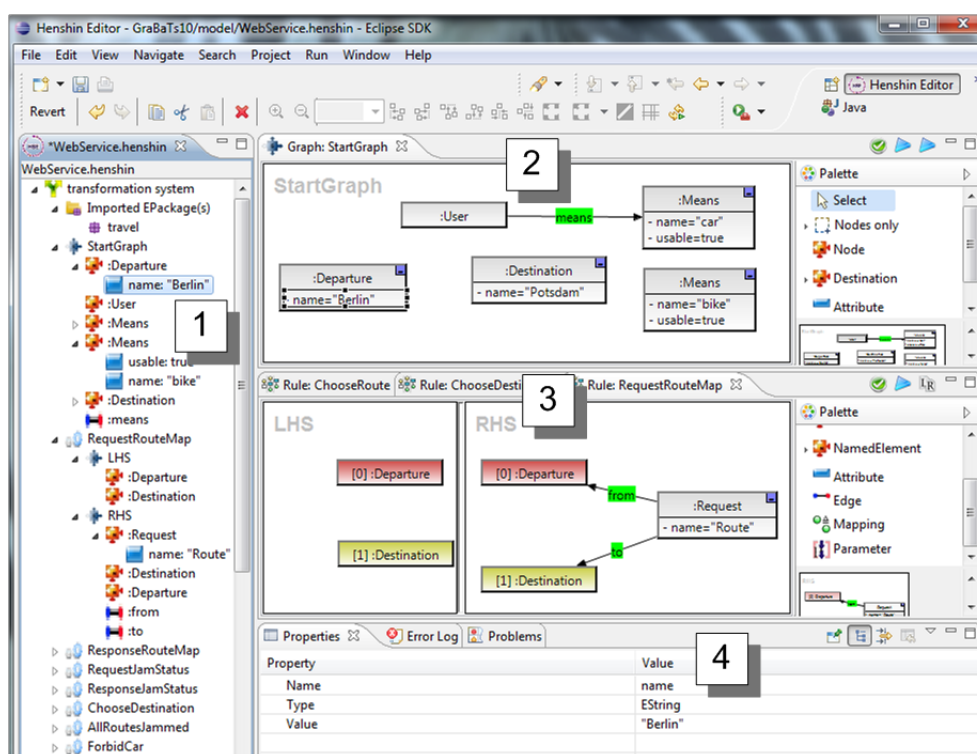
Figure 1: HENSHIN GUI with visual editors for graphs and rules.
