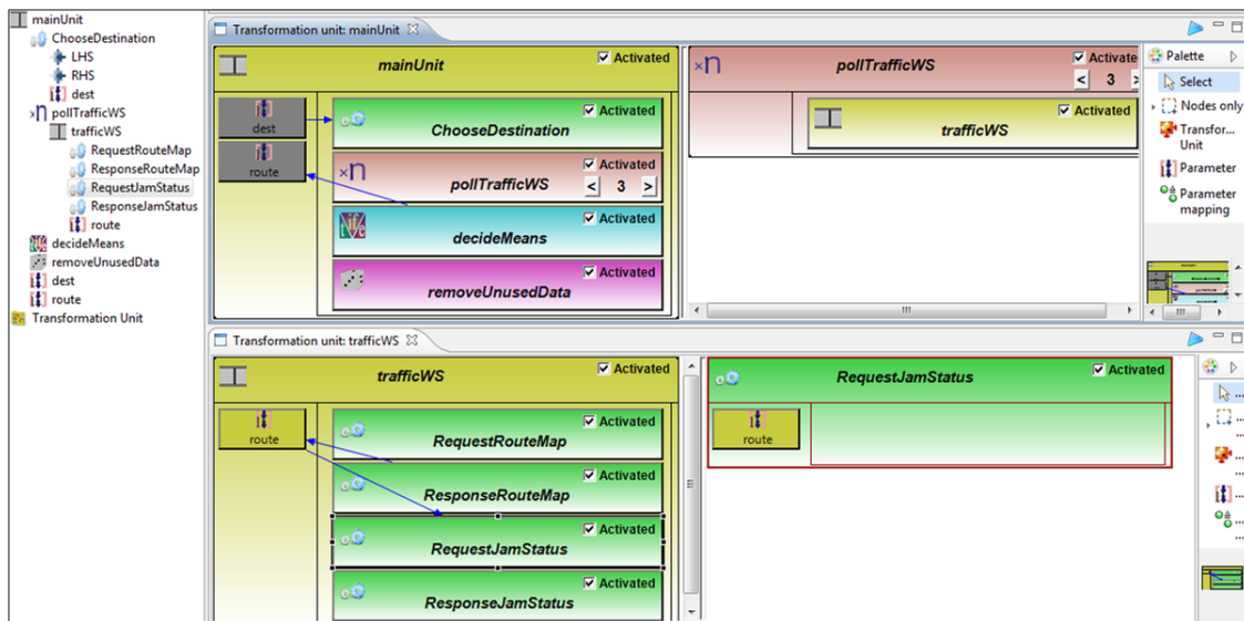
Figure 5: HENSHIN GUI with transformation unit editor
