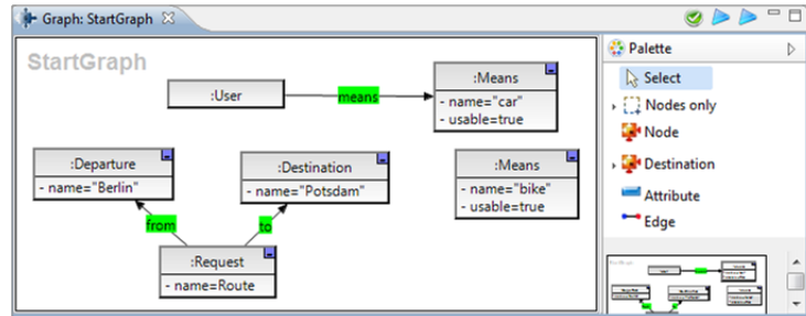
Figure 2: Transformed graph after applying rule RequestRouteMap
