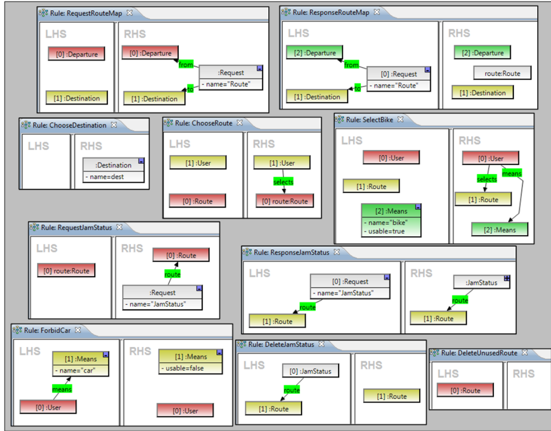
Figure 4: EMF model transformation rules for the Personal Mobility Manager
