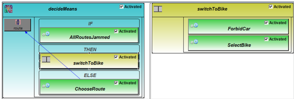
Figure 6: HENSHIN transformation unit decideMeans
