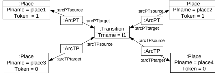
Fig. 7. AGG Instance Diagram over the P/T-Net Alphabet
