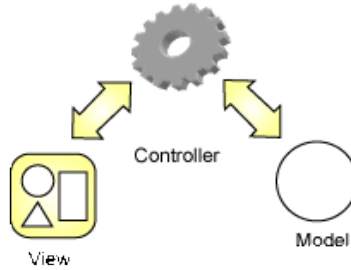
Fig. 2. Model-View-Controller
