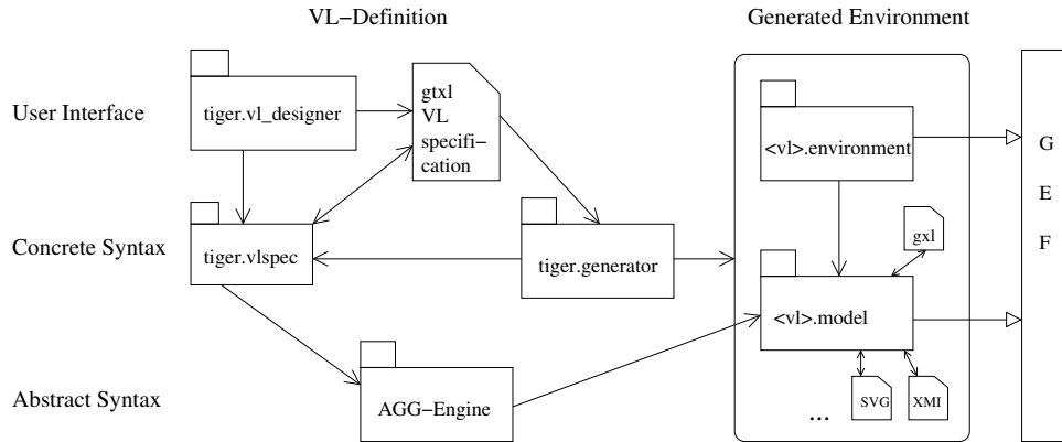
Fig. 3. Software Architecture
