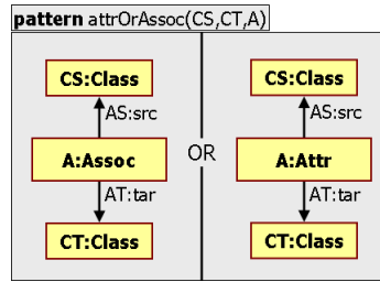
Fig. 26. Predefined helper graph patterns
