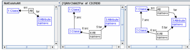
Fig. 13. Rule which collects attributes of subclasses in their parent classes
