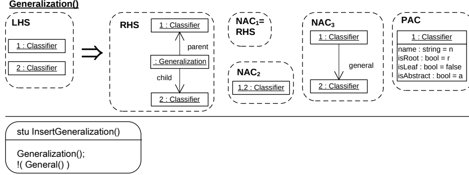
Fig. 3. Simple transformation unit for inserting a generalization
