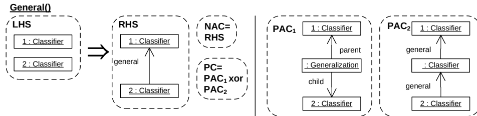
Fig. 4. Rule for creating transitive generalization relations
