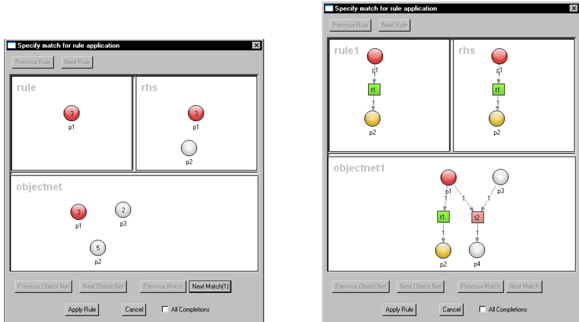
Figure 6: Match Dialogs: a) places with different markings and b) transitions with different pre- and post-domains
