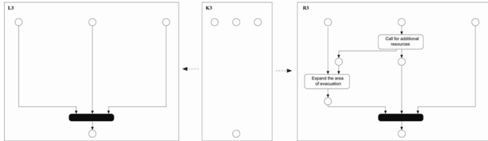
Fig. 4. Rule r_{expand}
