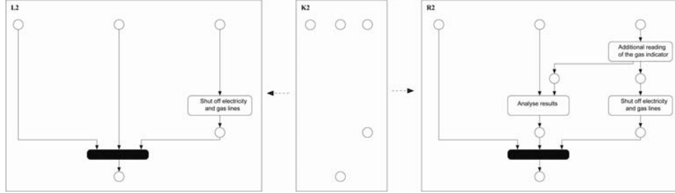
Fig. 3. Rule r_{analyse}
