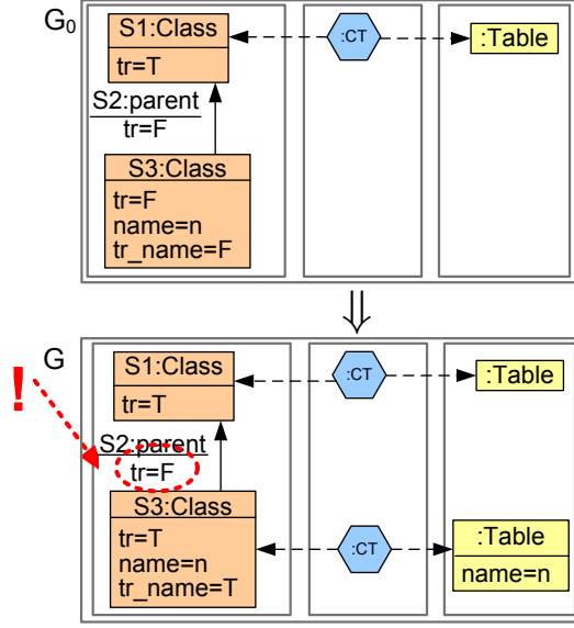
Figure 6: Step G_0 \xRightarrow{Class2Table_{FT}} G with misleading graph G
